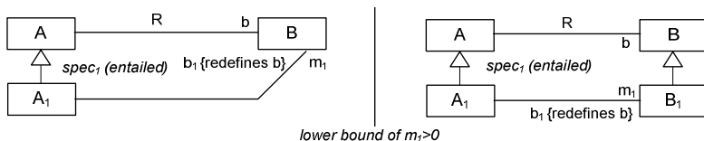
Fig. 4.2. Specialization constraint entailed by a multiplicity or a type and multiplicity redefinition
