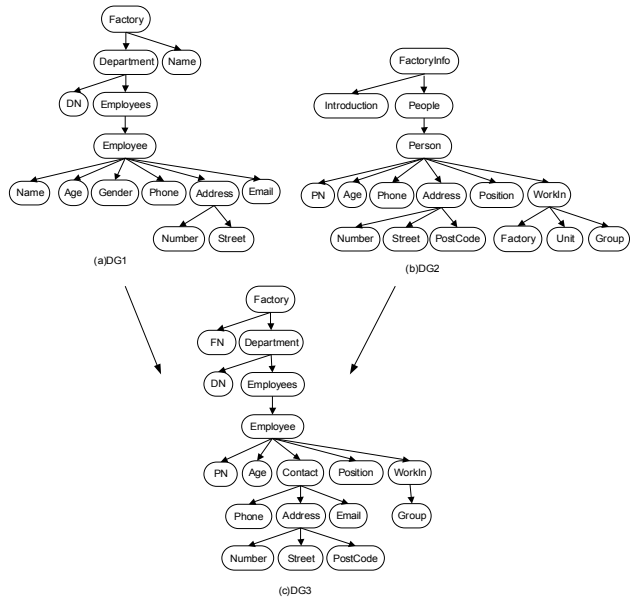
Fig. 1. DTD-Graphs of Doc_XML1, Doc_XML2 and Doc_XML3
