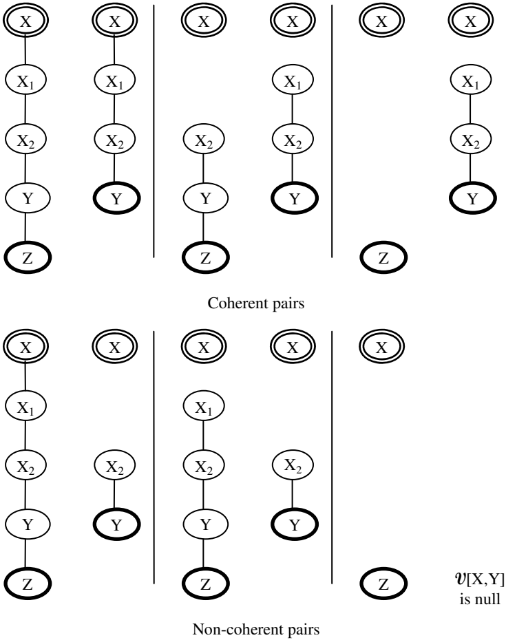
Fig. 5. Coherent property illustration
