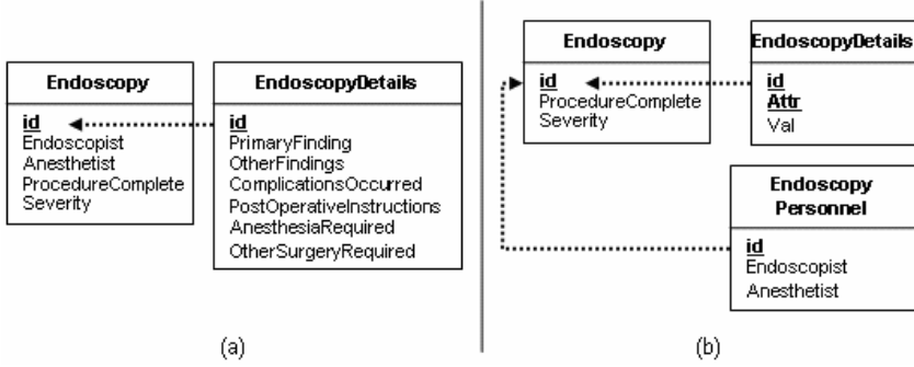
Fig. 4. The natural schema corresponding to Figure 3, before (a) and after (b) the application of a channel with operators \text{Unpivot}(\text{EndoscopyDetails}, \{\text{id}\}) and \text{VPartition}(\text{Endoscopy}, \{\text{id}\}, \{\text{ProcedureComplete}, \text{Severity}\}, \text{EndoscopyPersonnel})
