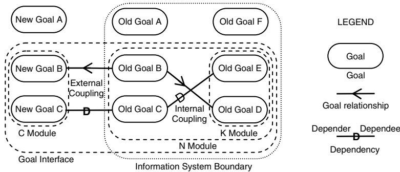
Fig. 2. Goal interface
