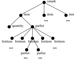
Fig. 3. Simplified XMARK document T_{xmark}
