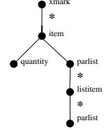
Fig. 4. Prefix tree of T_{xmark} , S_{xmark}
