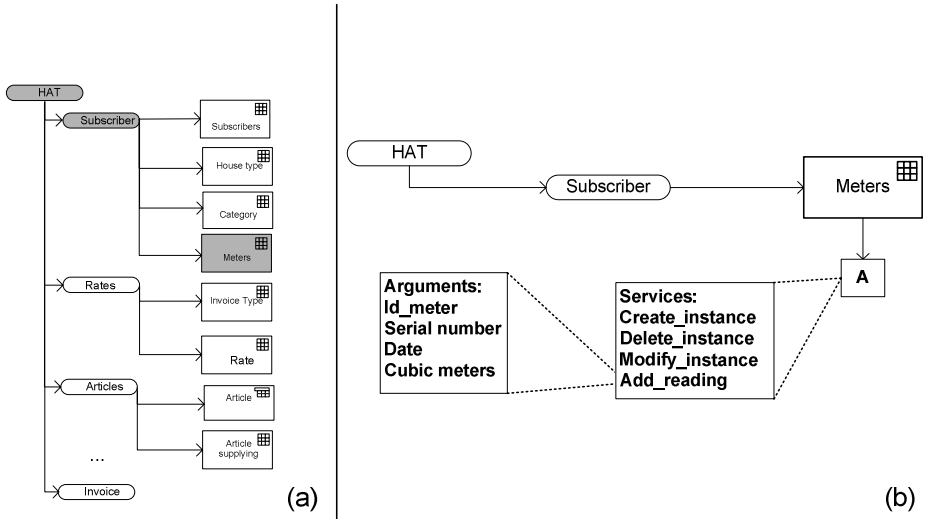
Fig. 4. Presentation Model
