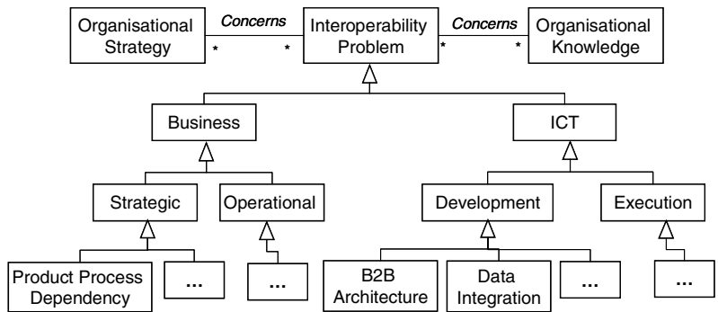
Fig. 4. Metamodel for interoperability problems classification
